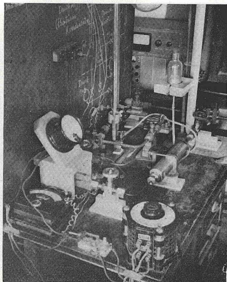
Apparatus for high pressure explosion, being manipulated at the right side of the steel wall protection— Laboratory of Physical Chemistry
