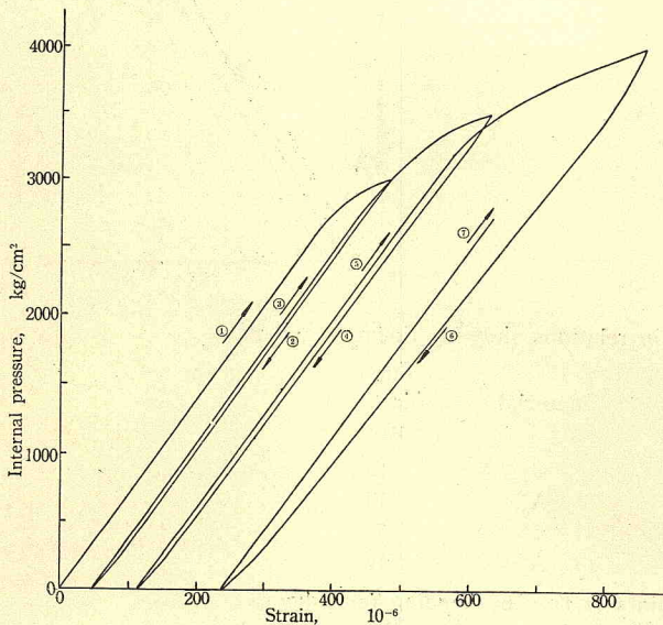
Fig. 6 Stress-strain relation showing stretching effect
