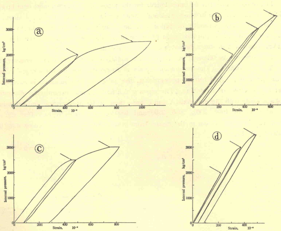
Fig. 5 Stress-strain relations showing linearity and flow
