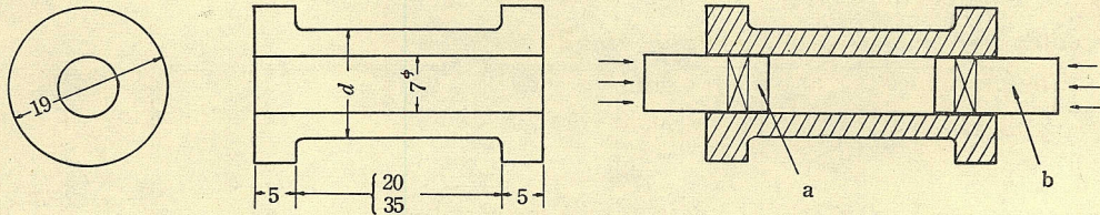
Fig. 2 Pipe and arrangement on testing a: Bridgman's plug b: piston
