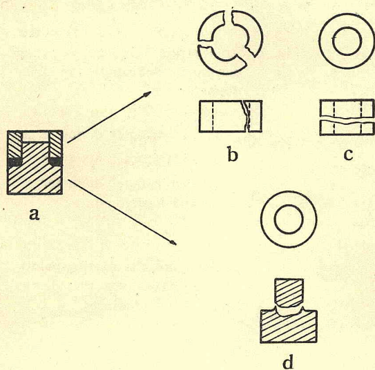
Fig. 8 Rupture of Bridgman's plug
